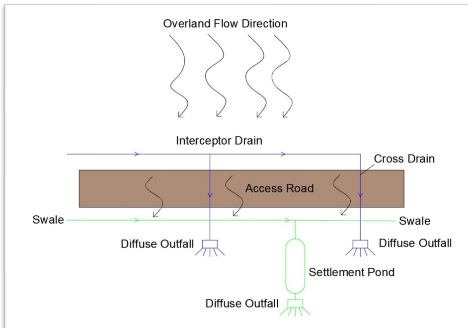
Plate 3-9: Drainage Diagram
