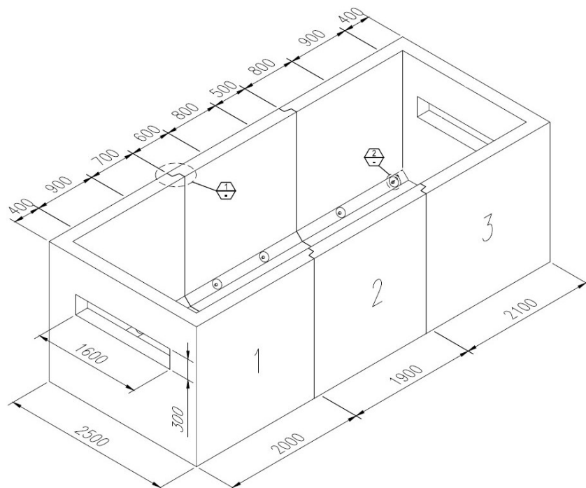
Figure 3-9: Eirgrid 110kV Single Circuit Joint Bay
